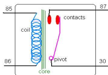
Figure 3 – Relay Symbol
